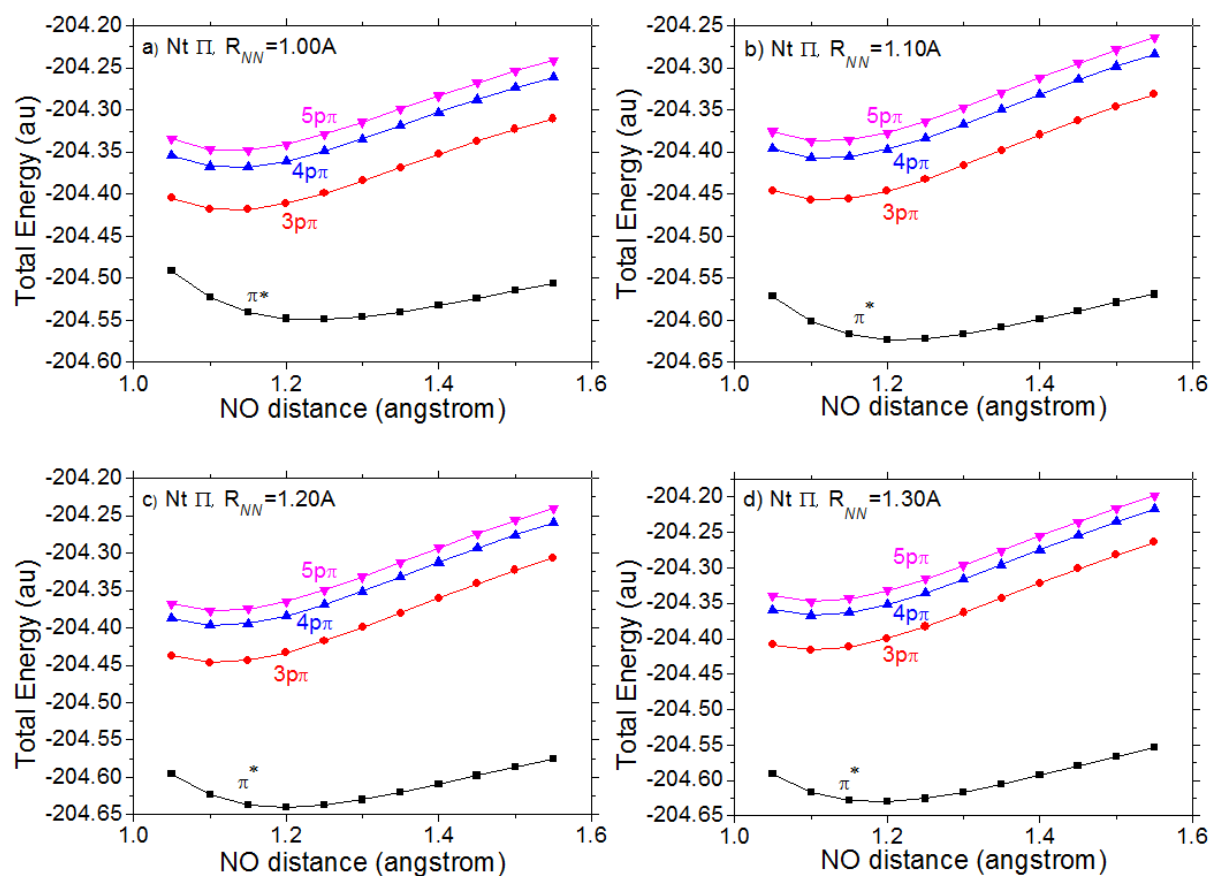
Figure 7. The 2D PESs of the low-lying N_t 1s excited states ( \pi^* and n\pi\pi ( n = 3-5 ) transitions) of N_2O in the R_{NO} coordinate for R_{NN} = 1.00, 1.10 [37], 1.20, and 1.30 \text{ \AA} .
