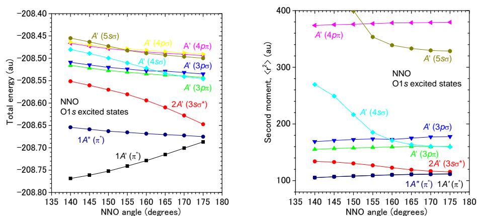
Figure 5. Potential energy curves (left) and second moments \langle r^2 \rangle (right) of the low-lying O 1s excited states of \text{N}_2\text{O} along the bending coordinate [29].
